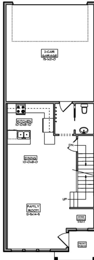
MAIN FLOOR 623 FinSqFt
