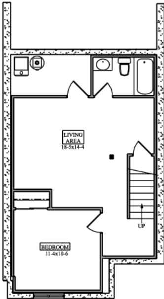
LOWER FLOOR 539 sqft (unfinished)
