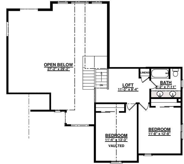
UPPER LEVEL FLOOR PLAN 576 sq ft
