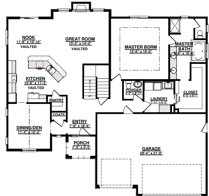
MAIN LEVEL FLOOR PLAN 1626 sq ft
