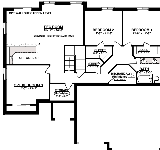
BASEMENT FLOOR PLAN 1628 sq ft
