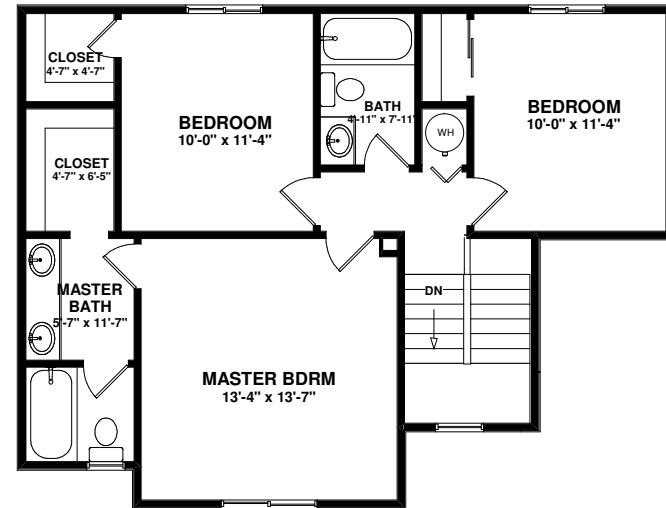
UPPER LEVEL FLOOR PLAN 680 sq ft
